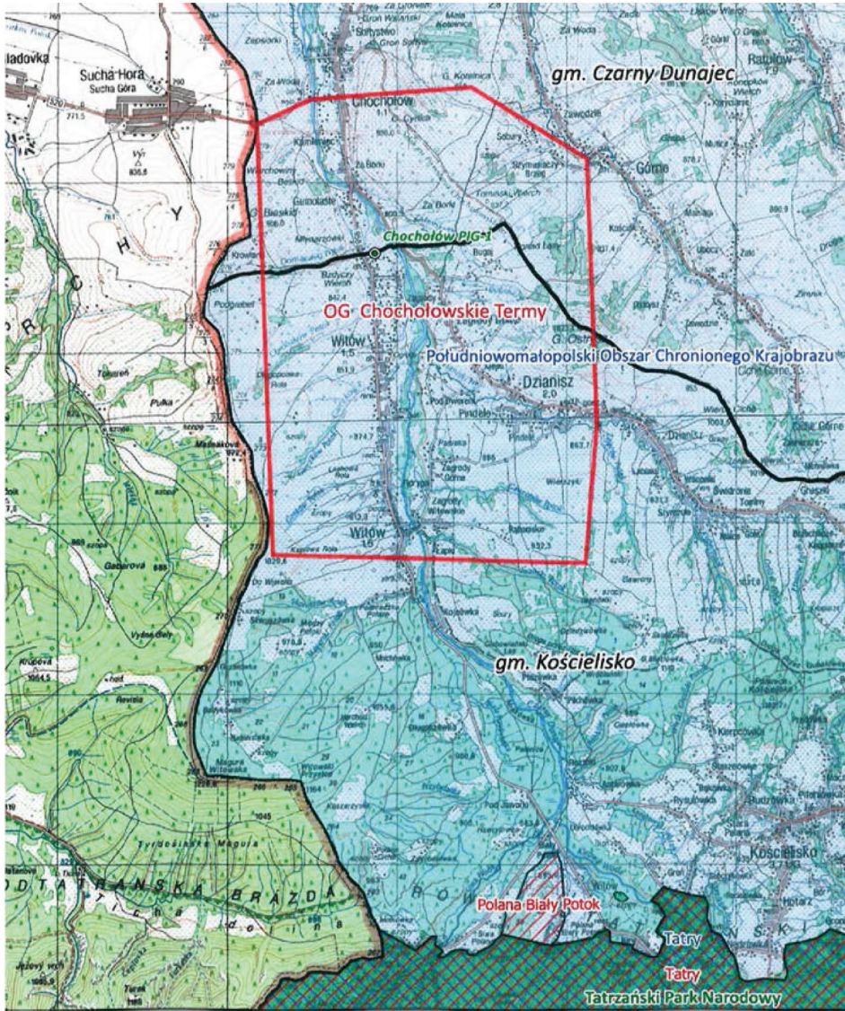
● Chochołów PIG-1 borehole ■ national parks ■ OSO areas Natura 2000 ■ mining area boundary ■ SOO areas Natura 2000 ■ landscape protected areas ■ administrative boundaries Source: own – modified (Bielec and Operacz 2018)
