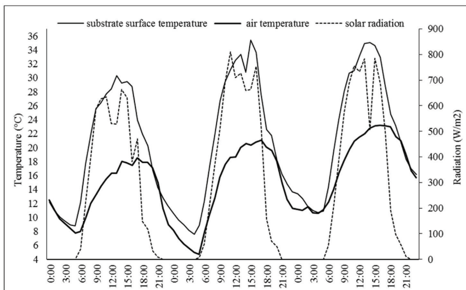
Figure 6. Solar radiation and the variations in air temperature and the substrate surface temperature in the lysimeter (11-13 June 2016)
