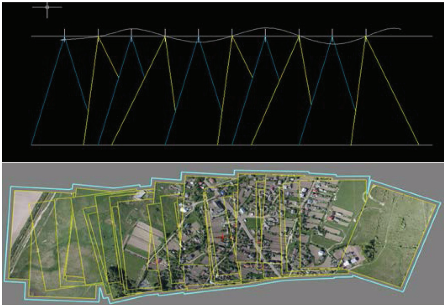
Figure 1. The effect of the pitch angle on the longitudinal overlapping of aerial photographs. The fluctuations of the pitch angle in accordance with the harmonic law (the frequency of oscillation is relatively low compared with the frequency of shooting) leads to a rhythmic instability of the longitudinal overlap.
