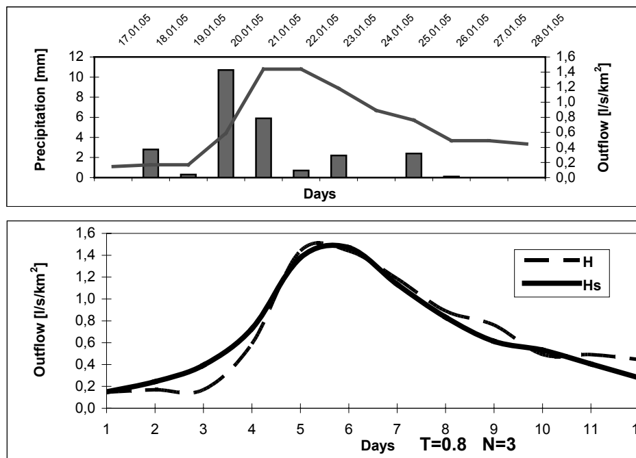
Figure 2. Example result of storm flow modeling in marshlands on the Promotion Forest Complex “Łasy Rychtałskie” (H – measured outflow, Hs – simulated outflow)
