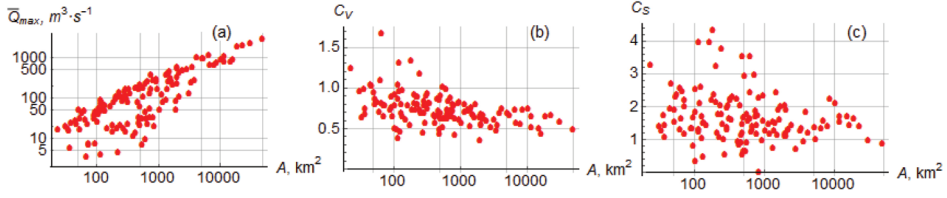
Figure 4. Basic characteristics of 138 time series of Q_{max} versus catchment area A : (a) mean, \bar{Q}_{max} , (b) coefficient of variation, C_v , and (c) skewness coefficient, C_s
