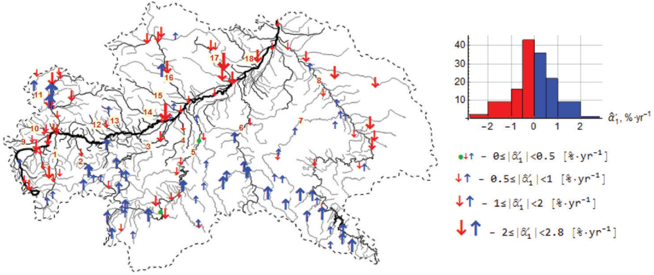
Figure 6. Spatial distribution of magnitude of 138 positive (↑) and negative (↓) relative slopes \hat{\alpha}'_1 divided into 8 classes (see histogram). Green dot (•) indicates two locations with estimated zero-slope.
