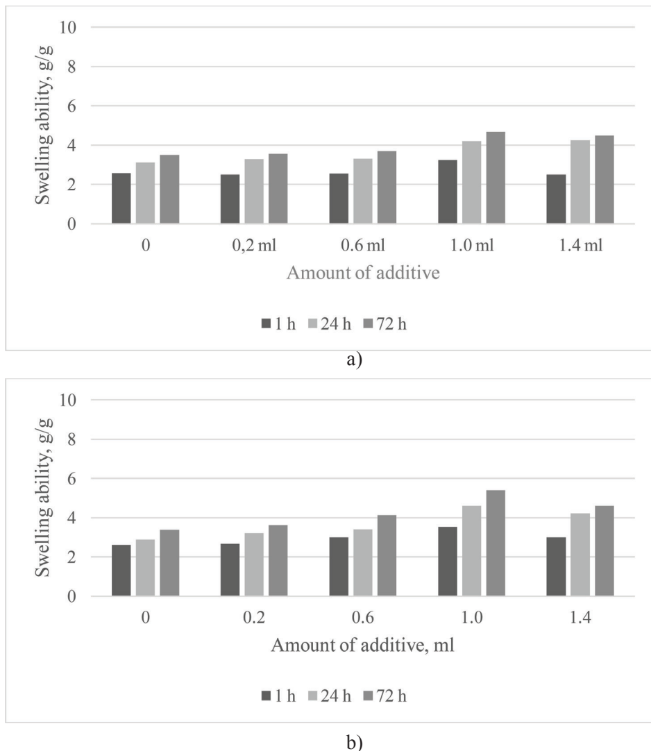
Figure 3. Swelling abilities of tested materials containing titanium dioxide in: a) SBF, b) distilled water.
