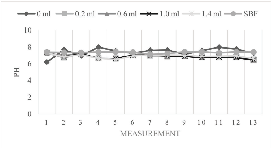
Figure 1. Changes of pH values of SBF solutions containing polymers containing: a) titanium, b) titanium dioxide.
