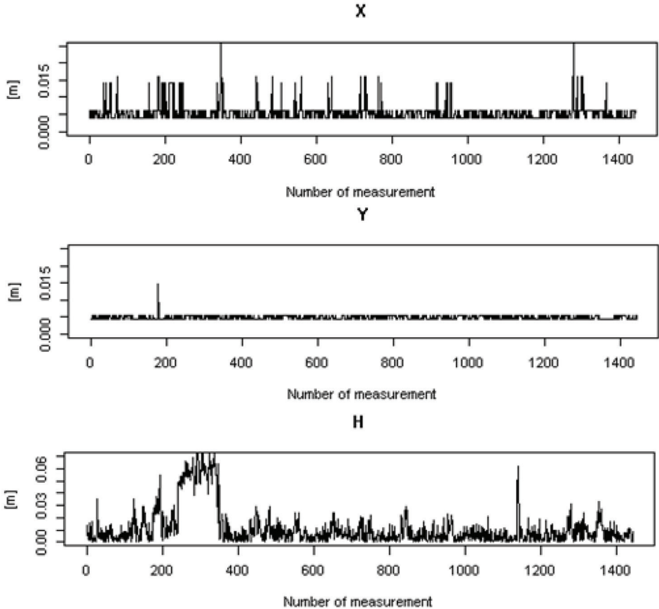
Figure 4. The absolute error of coordinates for subsequent VRSNET.PL results of measurements
