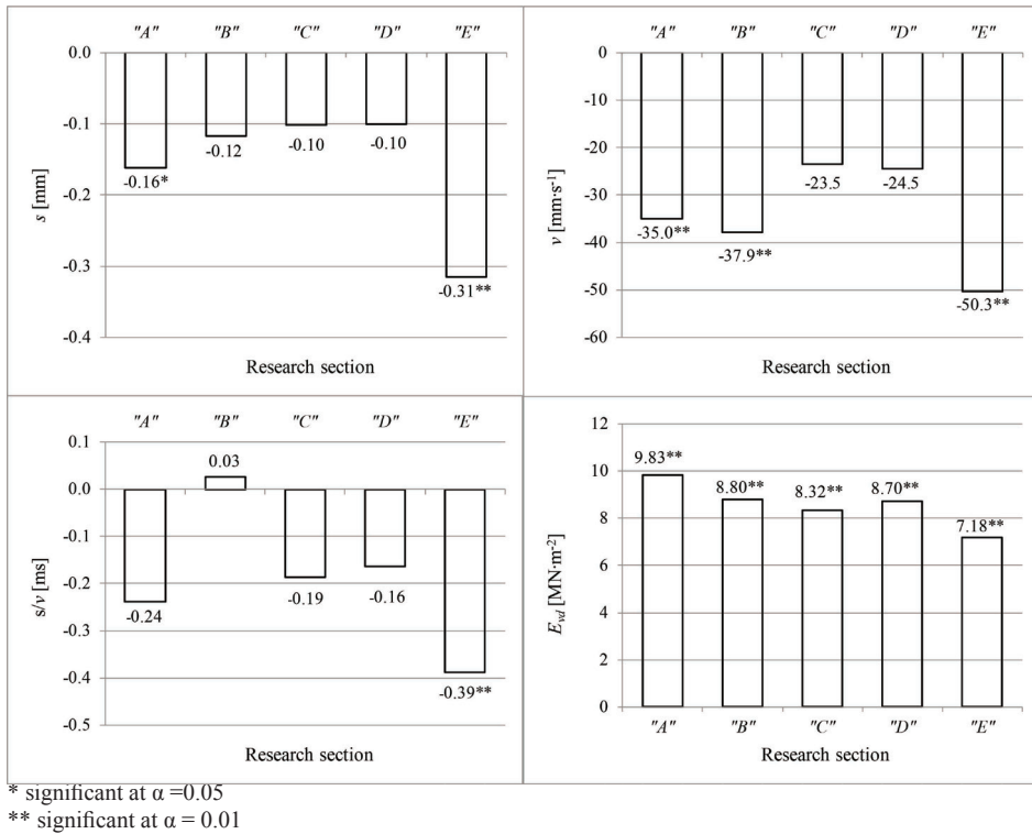
Figure 2. Differences in values of analysed bearing capacity parameters determined before and after the rainfall for four research sections (A – D) and the reference stretch (section E).
