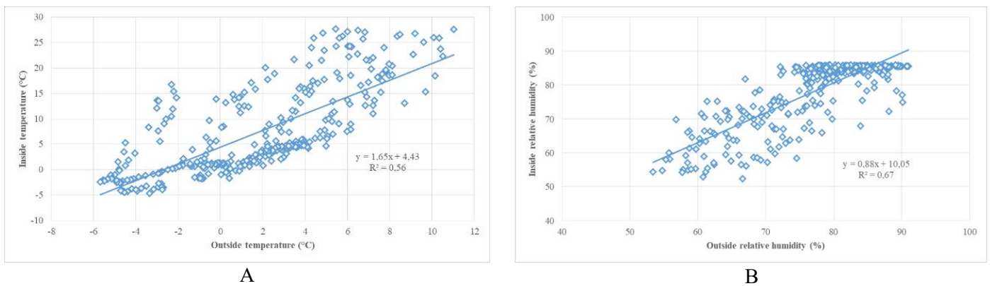
Figure 2. Relationship between (A) outside-inside temperature values and (B) outside-inside relative humidity values.
