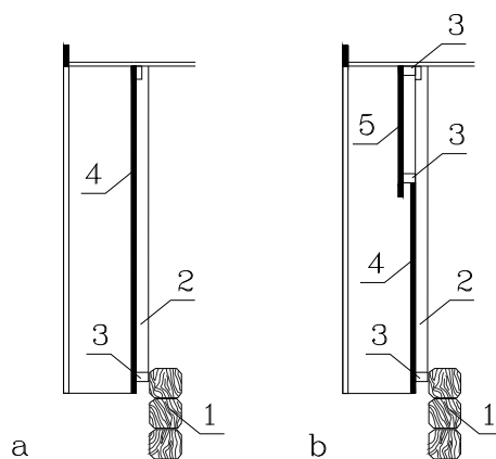
Fig. 15. Structure of an overhanging gable: a-a single overhang; b-a double overhang; 1-a corner-notched log construction, 2-a rafter, 3 - die squares, 4 - clapboards, 5 - upper clapboards
